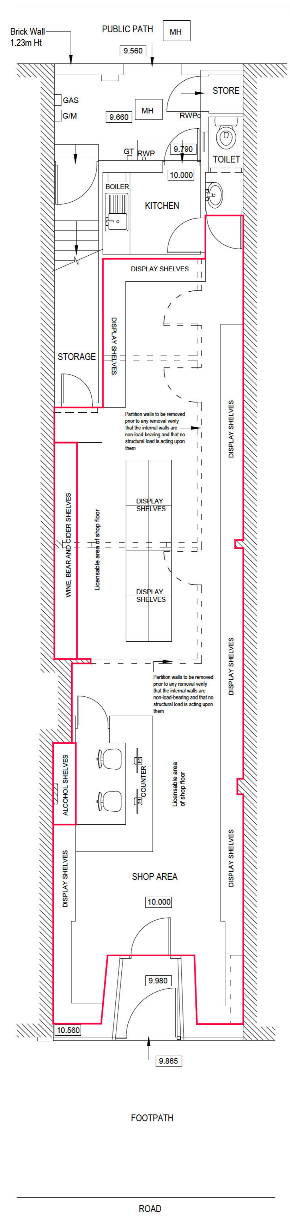
Ground Floor Plan Scale 1:50
